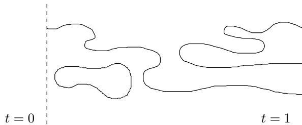
Figure 1.1: A one-dimensional cobordism
