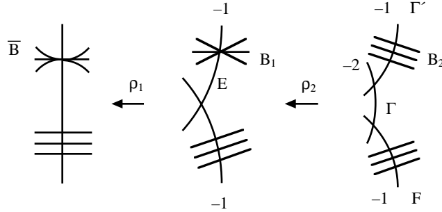
Figure 5.1: Producing reducible fibers ( g = 2, h = 1 ).
