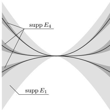
Figure 3.1: The supports of E_n .
