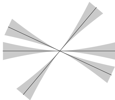
Figure 3.2: Different tangent lines.
