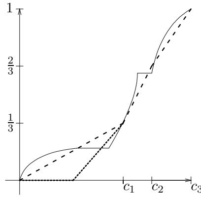
Figure 1: Reparametrization \psi —, homeomorphism \varphi - - and reparametrization \rho ···
