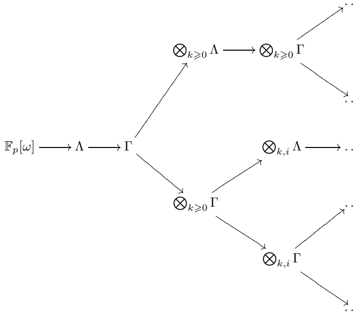
FIGURE 2. Schematic overview of iterated Tor-terms.
