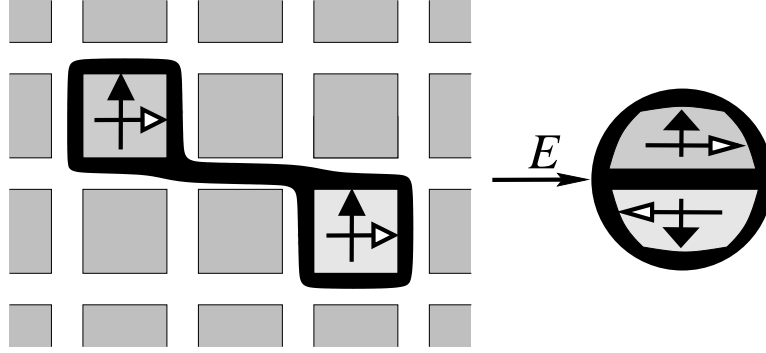
FIGURE 4.3. W and W' can be mapped almost isometrically into a cylinder. Rotation of this cylinder exchanges them and leaves all other pieces unchanged.
