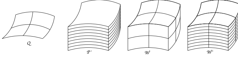
FIGURE 4.2. Schematic illustration of the partition Q , the partitions P' and W , and the common refinement W' .
