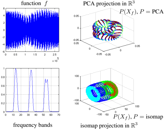
Fig. 2. Middle \gamma : PCA fails, but isomap recovers \Omega = \mathbb{T}^2 .
