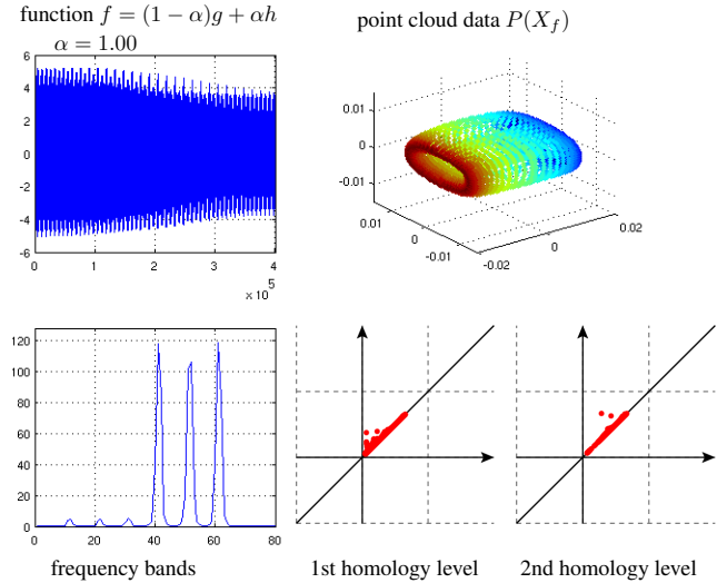
Fig. 6. f = h , and X_f \subset \mathcal{M} with \mathcal{M} homeomorphic to \mathbb{T}^2 .
