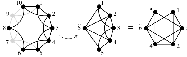
Figure 6.4: C_6^2 - v_1v_6 is a t -minor of C_{10}^2 - v_{10} .
