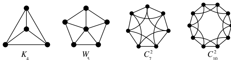
Figure 6.1: The forbidden t -minors.
