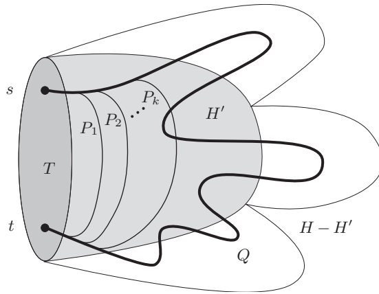
FIGURE 3. T -paths P_1, \dots, P_k that are disjoint outside Q
