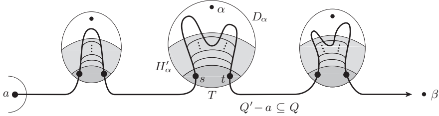
FIGURE 5. Modifying Q' - a into a path in G \cap G'
