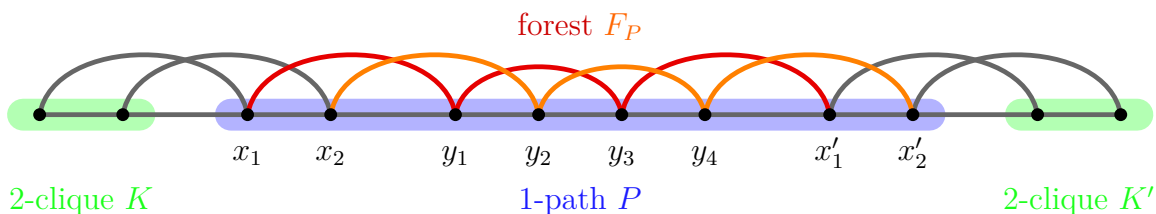
FIGURE 3.1. For k = 1 and \ell = 4 completing a 1-path P to a 2-path with a linear forest F_P consisting of two 3-edge paths.
