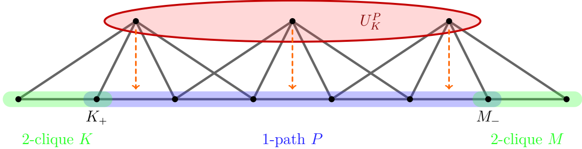
FIGURE 4.1. Building a 2-path Q for k = 1 that connects K and M by adding vertices from U_K^P to a 1-path P connecting K_+ and M_- at the indicated places.
