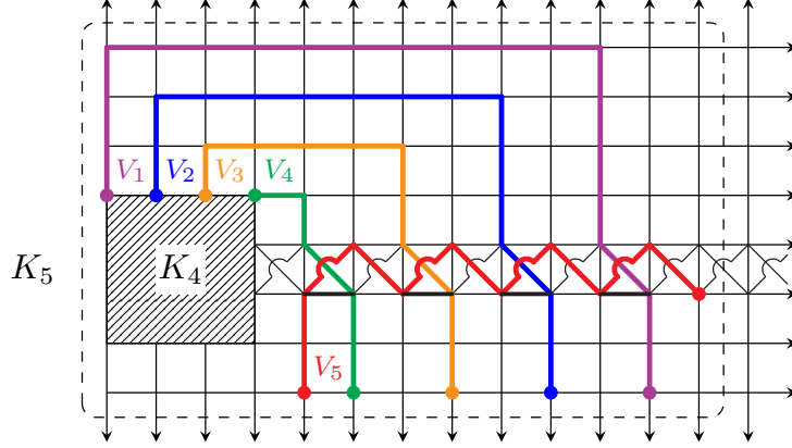
FIGURE 6.1. Sketch of a K_5 minor in a half-grid with all (i, 0)(i + 1, 1) and (i, 1)(i + 1, 0) edges. The branch paths E_{ij} between V_5 and the V_i 's are the thickened (i, 0)(i + 1, 0) edges.
