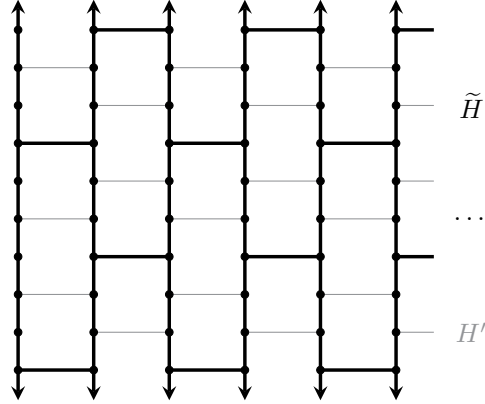
FIGURE 3.3. The black subdivision \tilde{H} of the hexagonal half-grid is a subgraph of the grey subdivision H' of the hexagonal half-grid.
