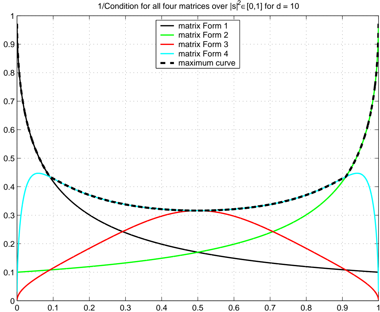
FIGURE 4.5. Inverse condition for all four matrices for d = 10 .
