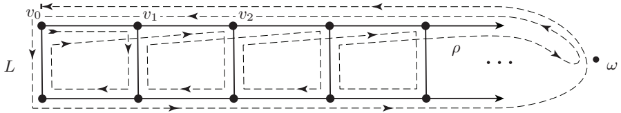
FIGURE 5.3. The loop \rho is not null-homologous
