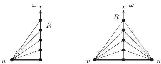
FIGURE 5.1. Should the fat edge sets be circuits?
