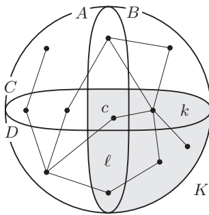
Figure 1: The cross-diagram \{(A, B), (C, D)\} with centre c and a corner K and its links k, \ell .
