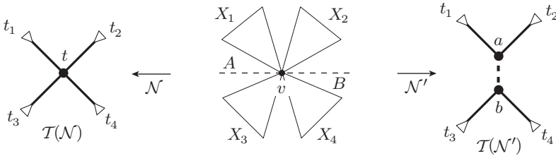
Figure 5: T' = \mathcal{T}(\mathcal{N}') has distinct nodes a, b whose parts in the tree-decomposition (\mathcal{T}', \mathcal{V}) coincide: V_a = \{v\} = V_b .
